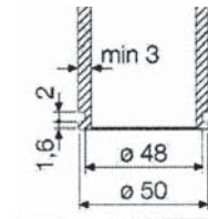
Detail Rohrende
